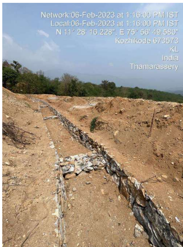
Garland drainage
